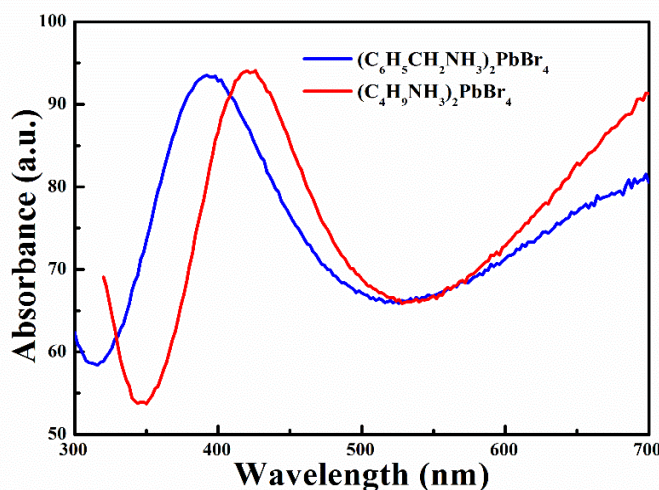
Figure 5. The absorption spectrum of the perovskite (\text{C}_4\text{H}_9\text{NH}_3)_2\text{PbBr}_4 (red curve) and (\text{C}_6\text{H}_5\text{CH}_2\text{NH}_3)_2\text{PbBr}_4 (blue curve).
