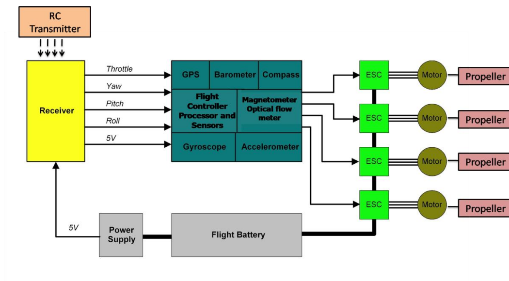
Figure 4.1 Block diagram
