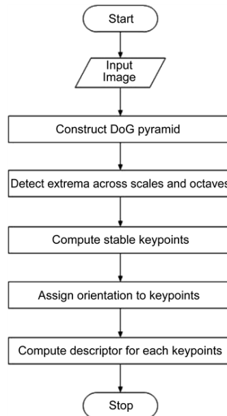
Fig 3: SIFT Algorithm
